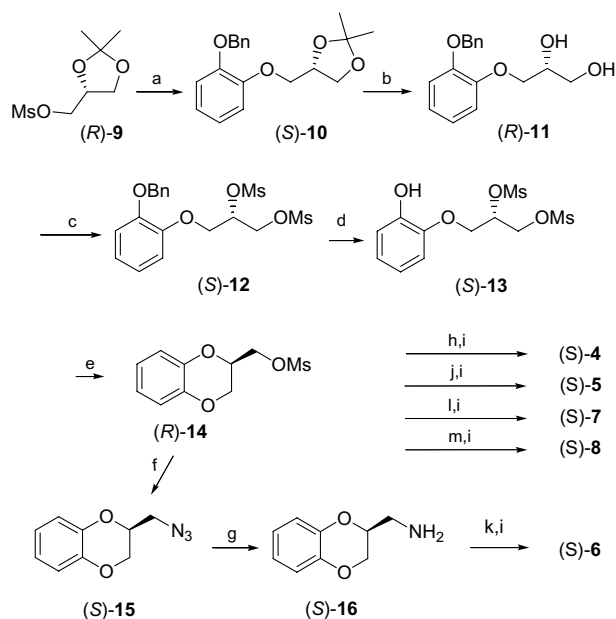
Scheme 1. Reagents and conditions: (a) 2-benzyloxyphenol, KOH, EtOH. (b) HCl. (c) MsCl, TEA. (d) H_2 -Pd/C, EtOAc, MeOH. (e) K_2CO_3 , acetone. (f) NaN_3 , DMF, H_2O . (g) hydrazine, PdO, MeOH. (h) 1-(2-aminoethoxy)naphthalene, 2-propanol. (i) HCl, EtOH. (j) 2-(2-aminoethoxy)naphthalene, 2-propanol. (k) 1-(2-bromoethoxy)-2-methoxynaphthalene, 2-methylpropanol. (l) 1-methoxy-2-(2-aminoethoxy)naphthalene, n -butanol. (m) 2-(2-aminoethoxy)-3-methoxynaphthalene, 2-propanol.
