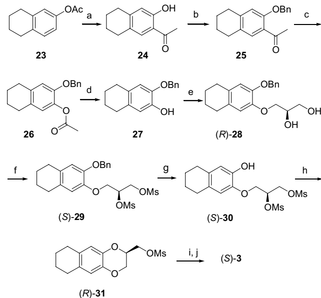
Scheme 3. Reagents and conditions: (a) AlCl_3 , 1,2-dichlorobenzene. (b) 2.5N NaOH, TBAB, benzyl bromide, DCM. (c) m -CPBA, CH_2Cl_2 . (d) MeOH, 2.5N NaOH. (e) ( R )- 9 , KOH, EtOH; MeOH, HCl. (f) MsCl, TEA, DCM. (g) H_2 -Pd/C, EtOAc. (h) K_2CO_3 , acetone. (i) 2-(2,6-Dimethoxyphenoxy)ethylamine, 2-propanol. (j) HCl, EtOH.
