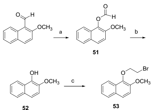
Scheme 5. Reagents and conditions: (a) m -CPBA, CH 2 Cl 2 . (b) LiAlH 4 , THF. (c) Dibromoethane, NaH, THF, DMSO.
