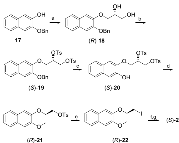
Scheme 2. Reagents and conditions: (a) ( R )- 9 , NaOH, EtOH; HCl. (b) TsCl, Py. (c) H_2 -Pd/C, EtOAc. (d) K_2CO_3 , acetone. (e) NaI, acetone. (f) 2-(2,6-dimethoxyphenoxy)ethylamine, 2-propanol. (g) HCl, EtOH.
