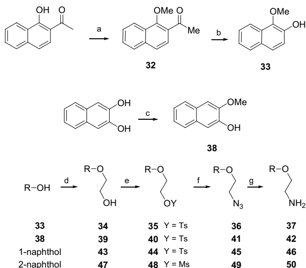
Scheme 4. Reagents and conditions: (a) MeI, KOH, DMSO. (b) m -CPBA, CH 2 Cl 2 ; H 2 SO 4 , MeOH. (c) Me 2 SO 4 , Me 3 COK, 2-methoxyethanol. (d) Ethylene carbonate, K 2 CO 3 , toluene or DMF. (e) TsCl and Py or MsCl and Et 3 N. (f) NaN 3 , DMF. (g) Hydrazine, PdO, MeOH.
